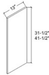
Wall End Panel (3/4" Thickness) WEP18mmx13"x31-1/2" WEP18mmx13"x41-1/2"
