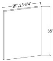
Base End Panel (3/4" thickness) BEP18mmx25"x35" BEP18mmx25-3/4"x35"
