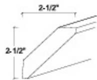
Crown Moulding CM8-F
