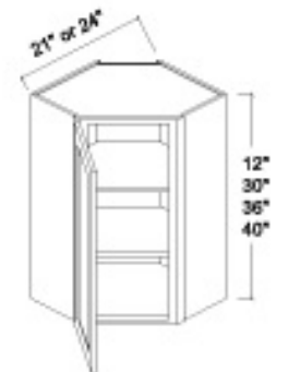
WDC2130/WDC2136/WDC2140 WDC2430/WDC2436/WDC2440 WDC2412
